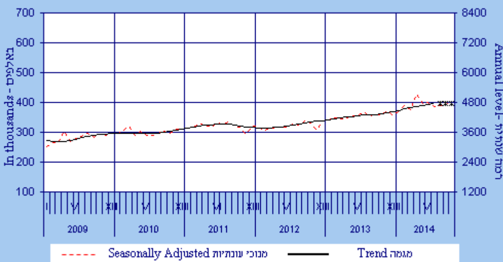
Figure 2. Departures abroad of Israelis by air
